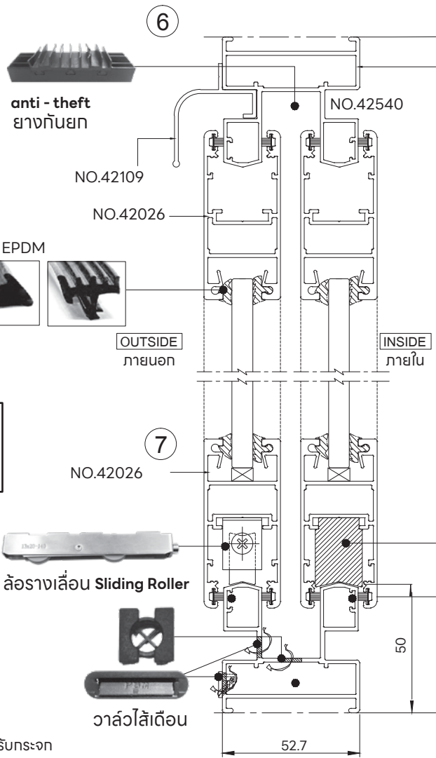
SECTION-B VERTICAL SECTION DETAIL FRAME WIDTH 50 mm.
