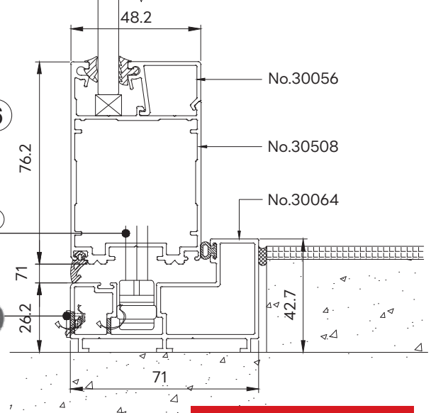
SECTION-B VERTICAL SECTION DETAIL
