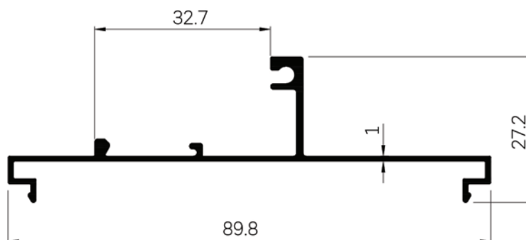
42560 WT : 0.452 Kg./m.
